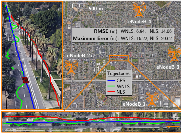
Fig. 7. Experimental results for positioning with LTE SSS signals in downtown Riverside, California, using: (i) WNLS estimator whose weights were calculated to (12) and (ii) NLS estimator. The position errors are calculated with respect to the GPS solution. Image: Google Earth.
